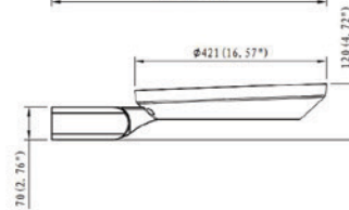
Side entry mounting
