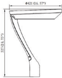
Single strut mounting
