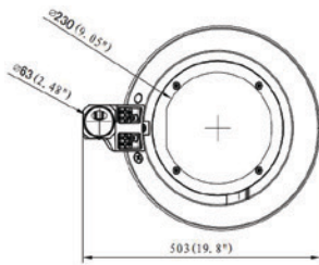
Single strut mounting
