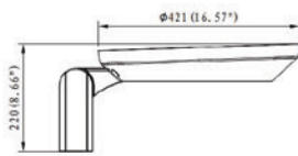
Post top mounting
